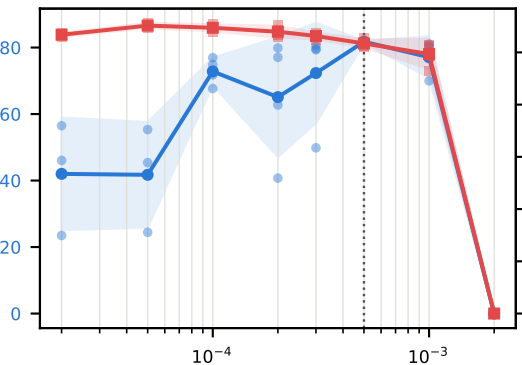
LoRA+wd
